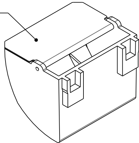
ITEM 2 SP-21AX WATER TANK ASSY
