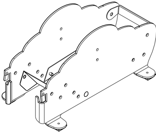
ITEM 1 SP-1XXX FRAME AND FOOT ASSY
